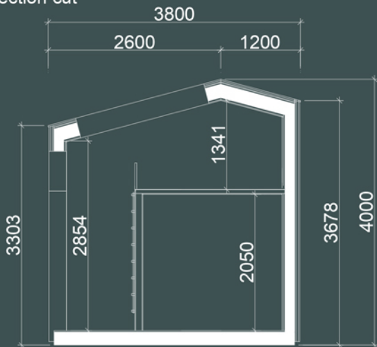
Section cut
